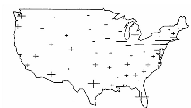
Figure 4 Gaining and losing states based on the marginals of a 48 by 48 migration table.
