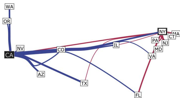
Figure 11 Immigration to California and New York
