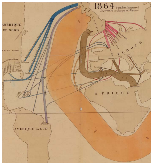
Figure 3 Minard’s 1864 flow map of cotton brut imports
