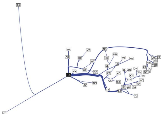
Figure 10 California migrations flow map
