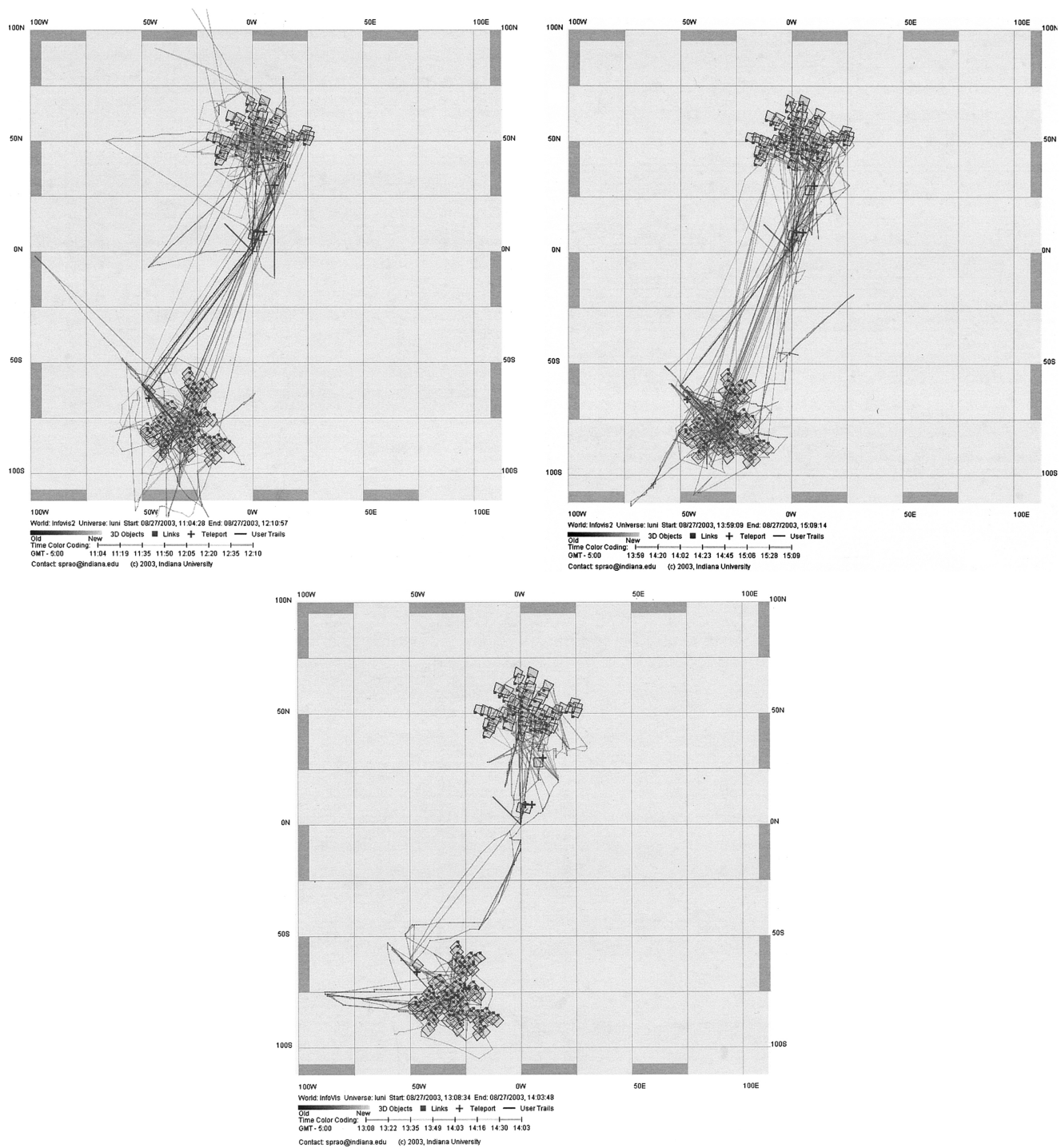
Figure 7. Group activity maps: Group 2 (upper left), Group 3 (bottom), and Group 4 (upper right).
