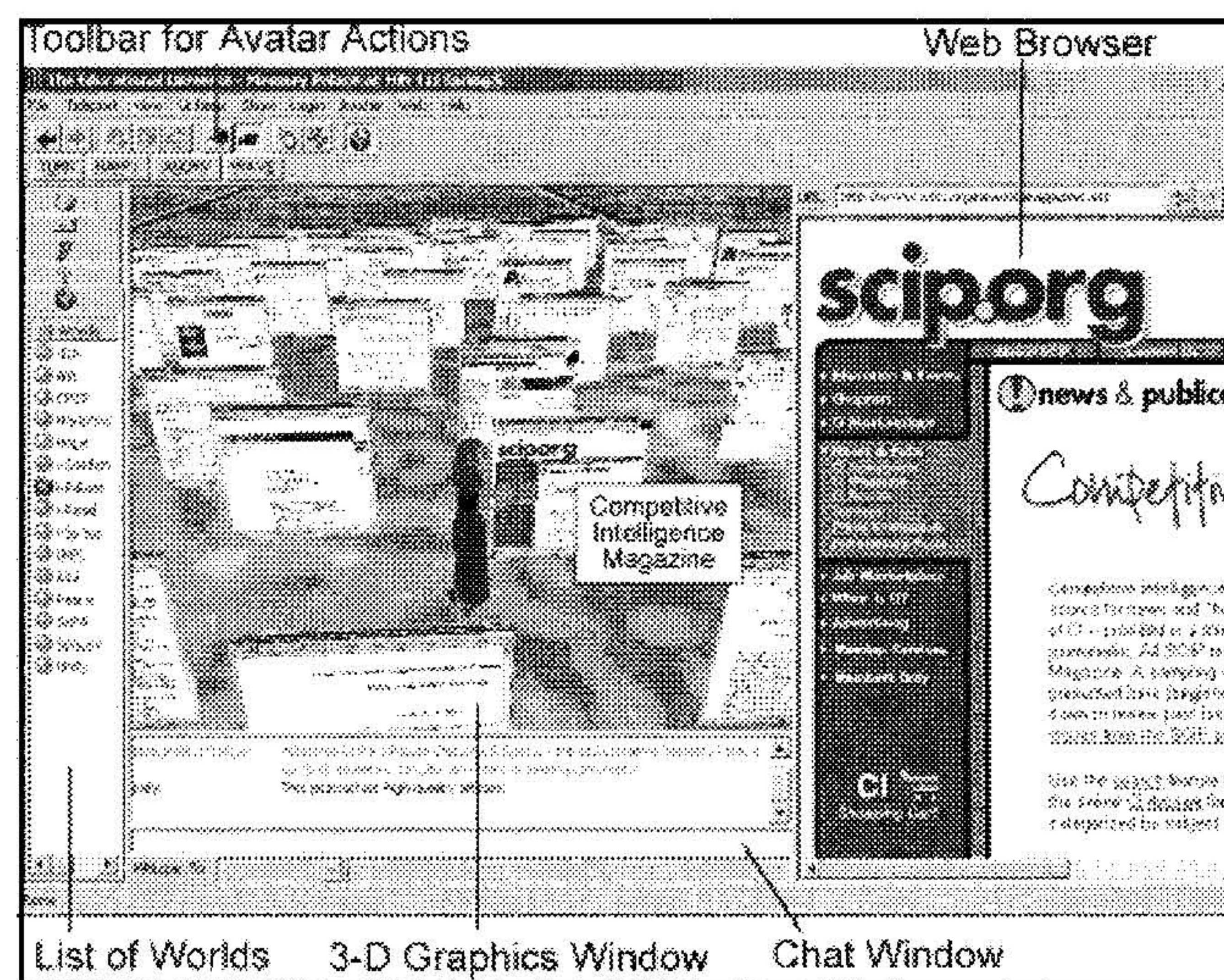
Figure 1. Desktop Interface to the SLIS Document Space
